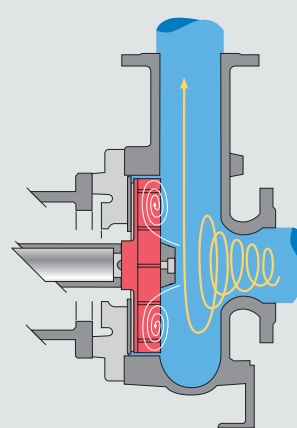
Totally recessed impeller
